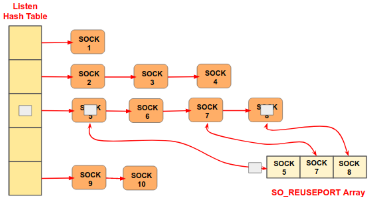
Figure 2.4: SO_REUSEPORT
