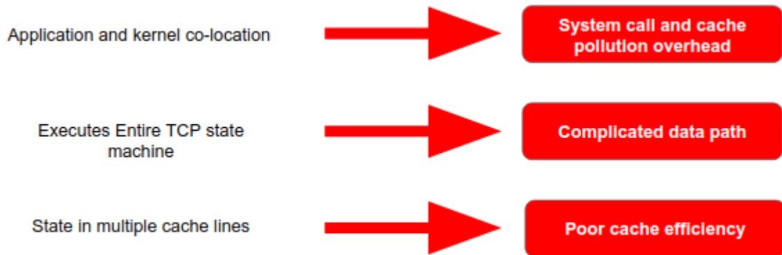
Figure 3.23: Issues TAS identifies
