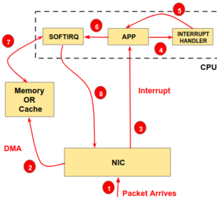
Figure 2.1: Linux network stack
