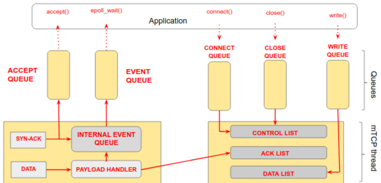
Figure 3.16: mTCP Implementation
