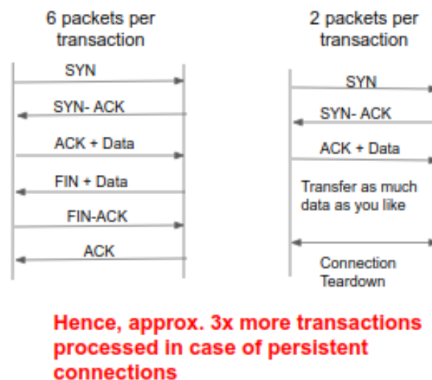
Figure 3.34: Short Connections
